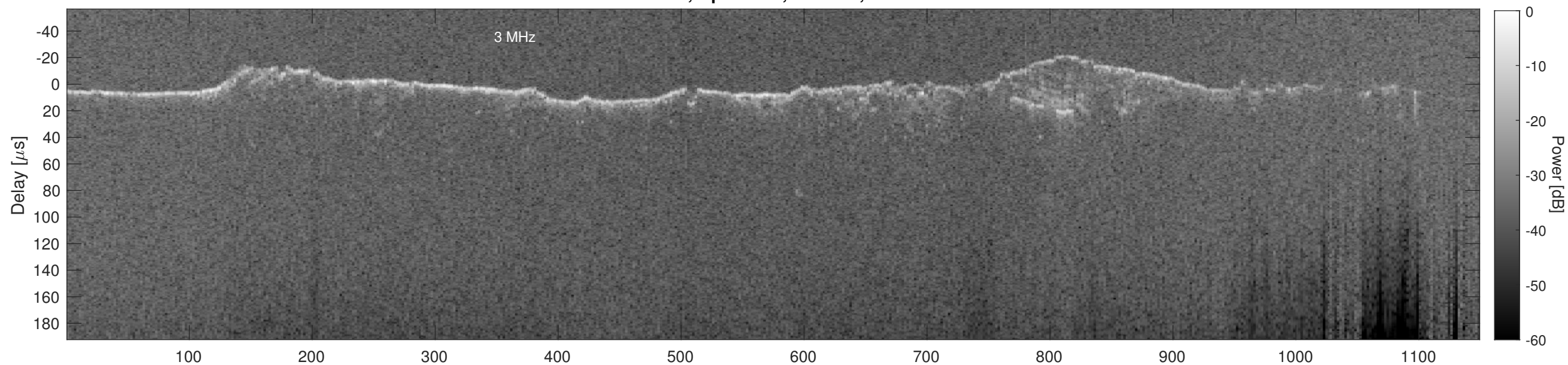
Orbit 13049, Cluttergram
