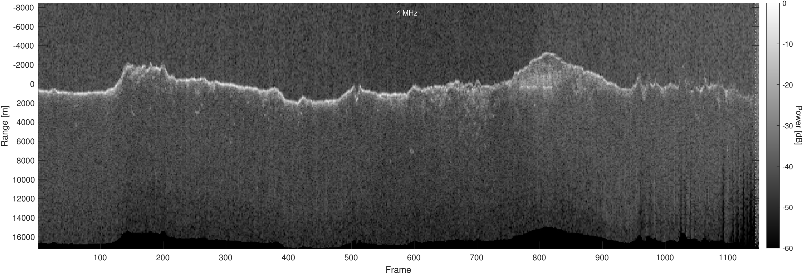
Orbit 13049, Optimized, Window, Depth-Corrected, Channel 2
