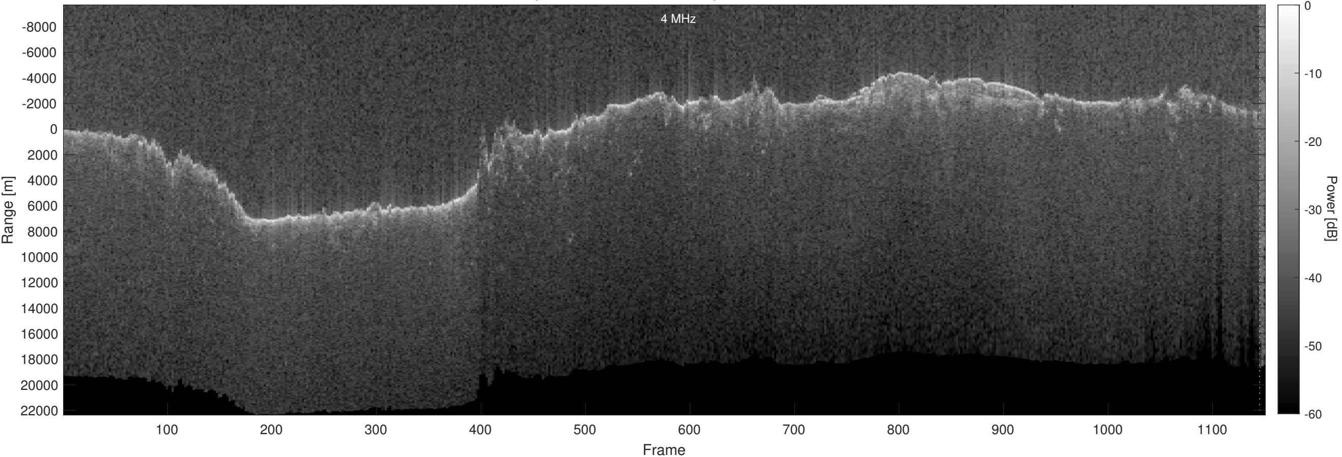
Orbit 13051, Optimized, No Window, Depth-Corrected, Channel 2
