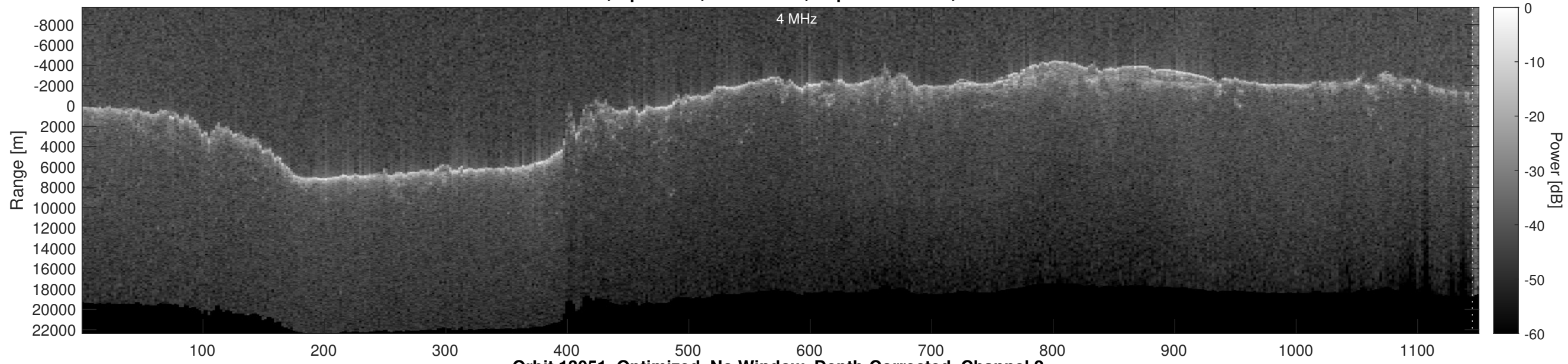
Orbit 13051, Optimized, No Window, Depth-Corrected, Channel 2
