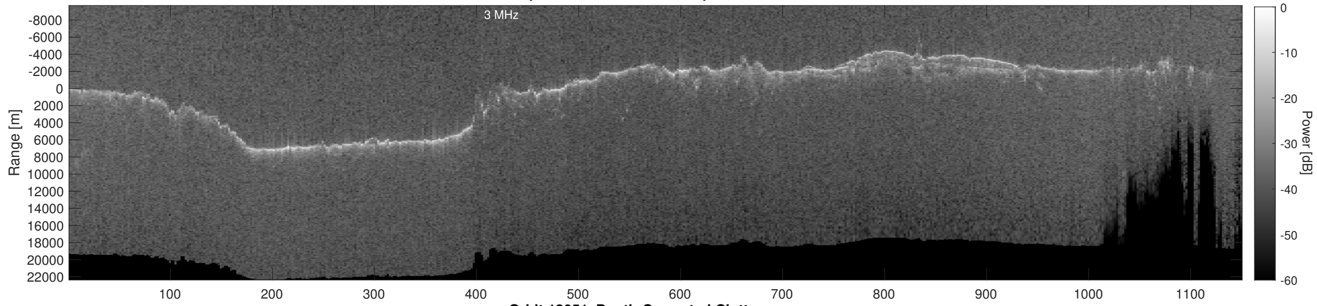
Orbit 13051, Depth-Corrected Cluttergram
