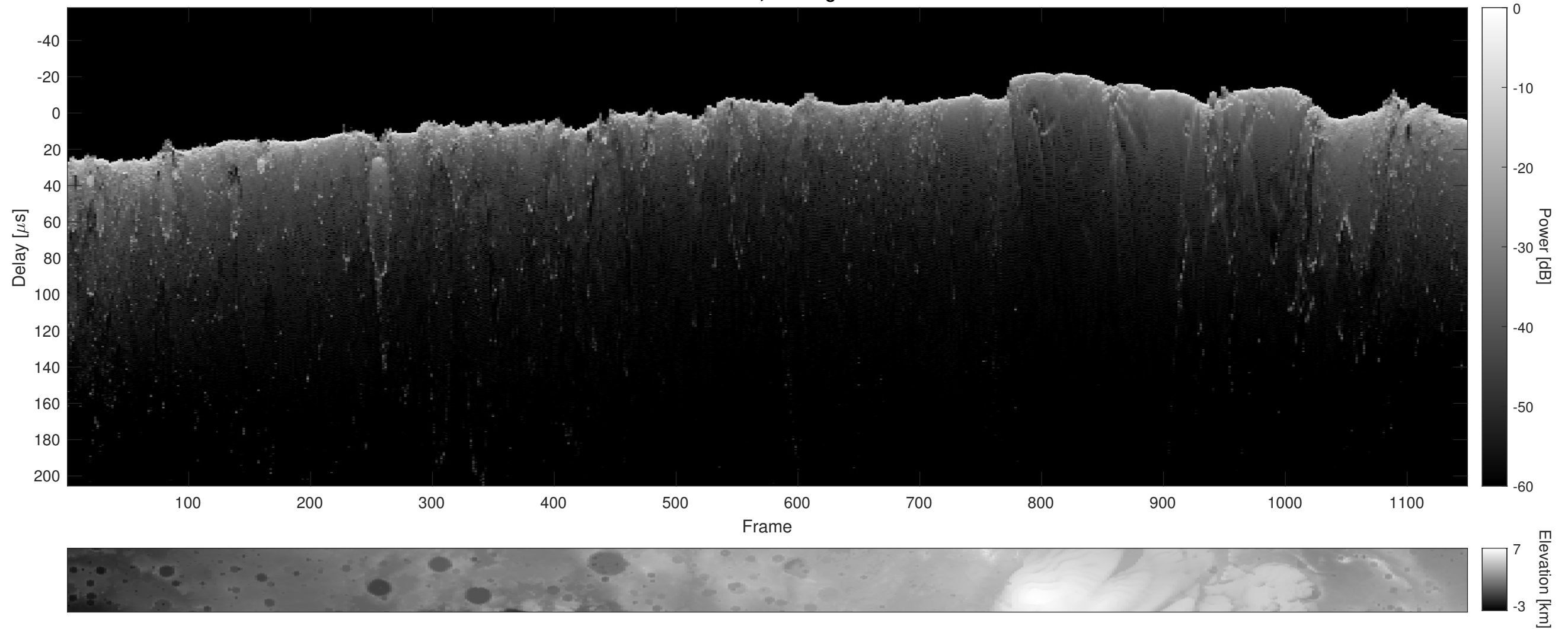
Orbit 13052, Cluttergram
