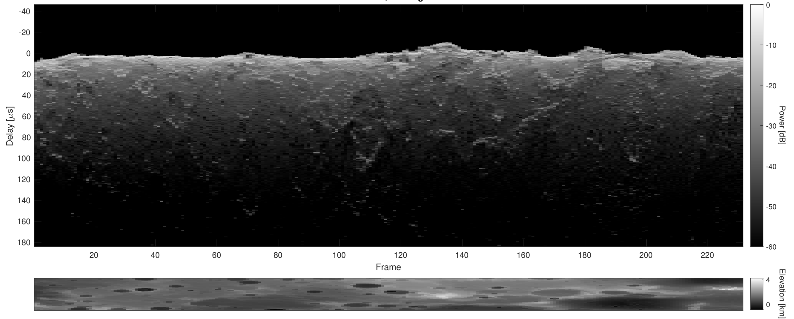
Orbit 13057, Cluttergram
