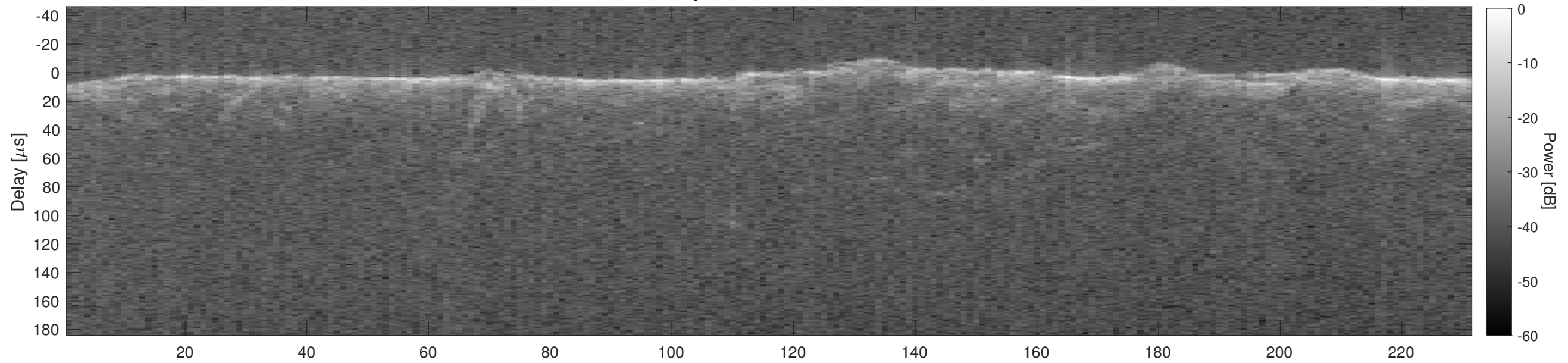
Orbit 13057, Cluttergram
