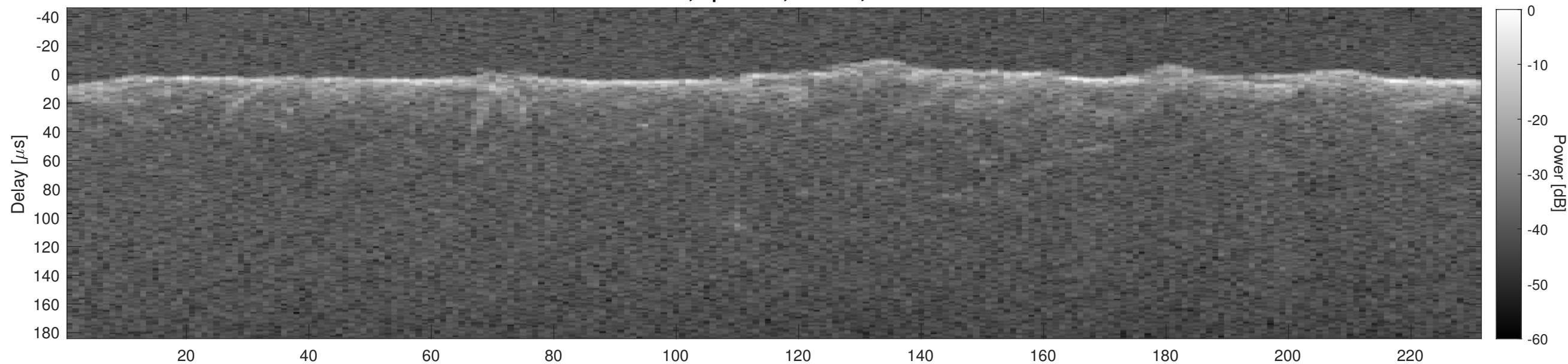
Orbit 13057, Cluttergram
