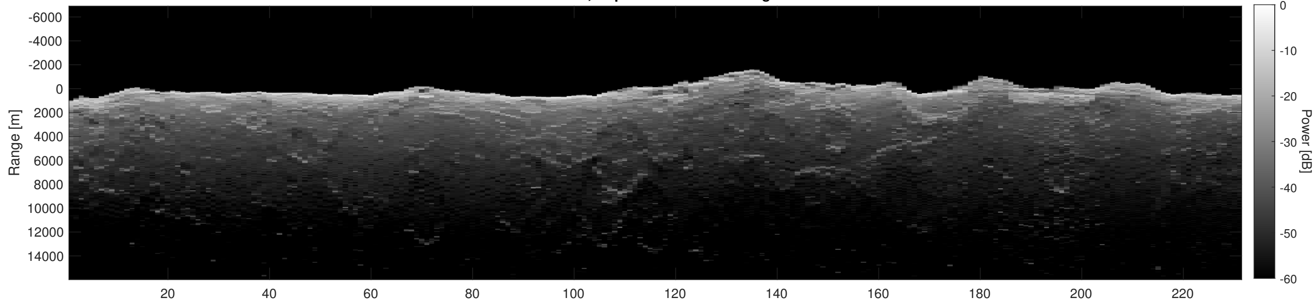
Orbit 13057, Depth-Corrected Cluttergram
