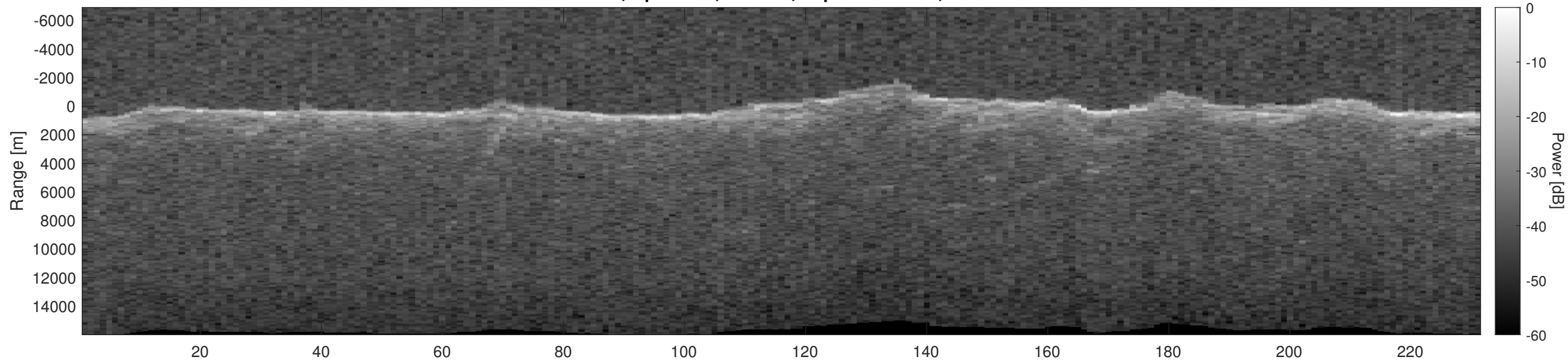
Orbit 13057, Optimized, Window, Depth-Corrected, Channel 2
