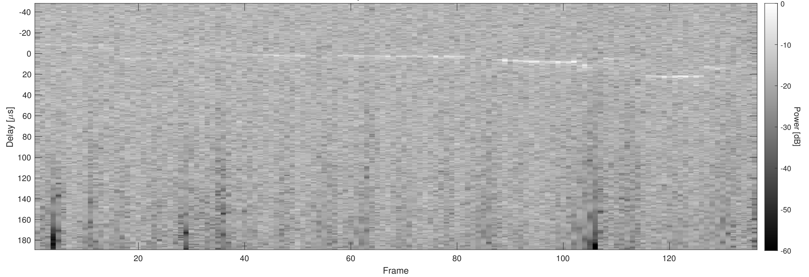
Orbit 13058, Optimized, No Window, Channel 2
