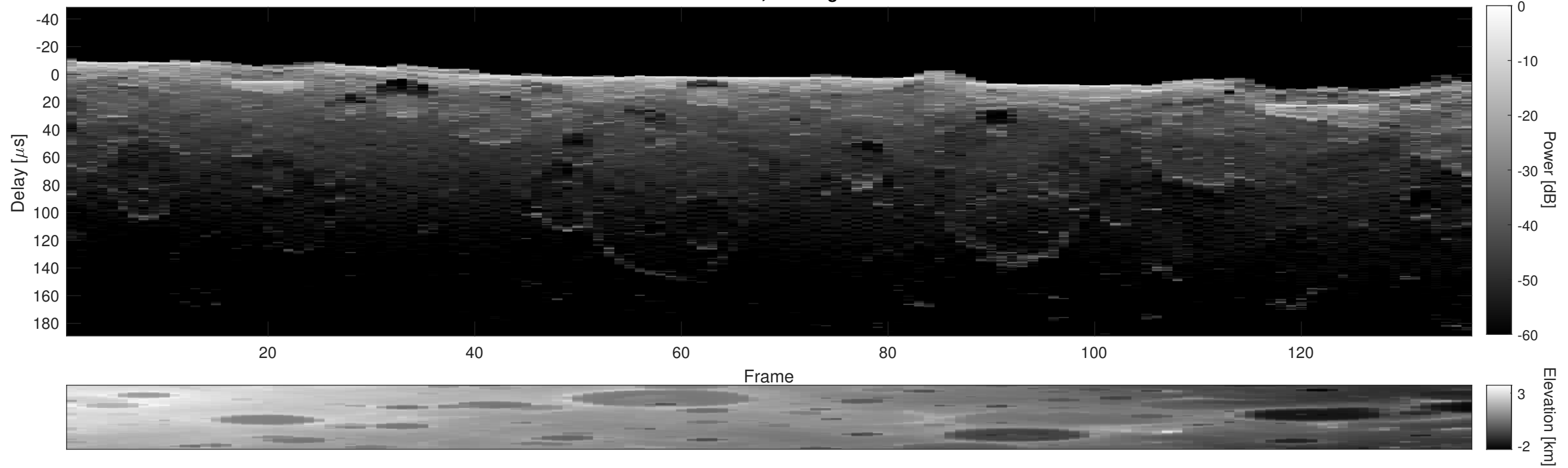
Orbit 13058, Cluttergram
