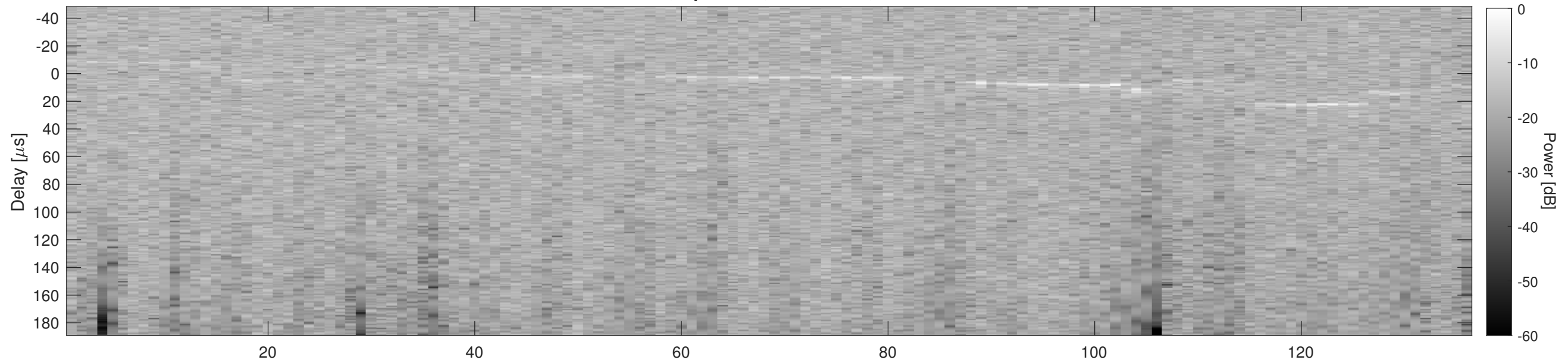
Orbit 13058, Cluttergram
