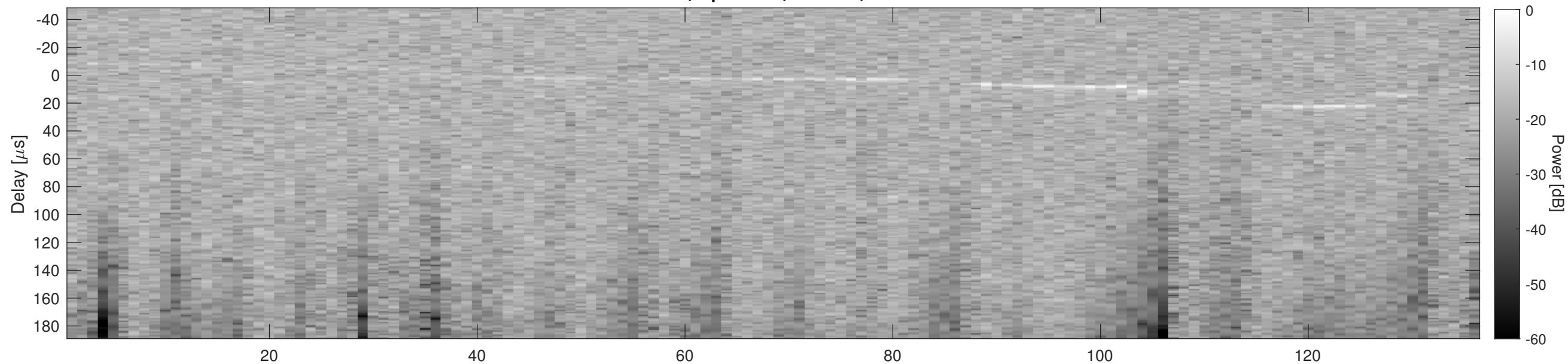
Orbit 13058, Cluttergram
