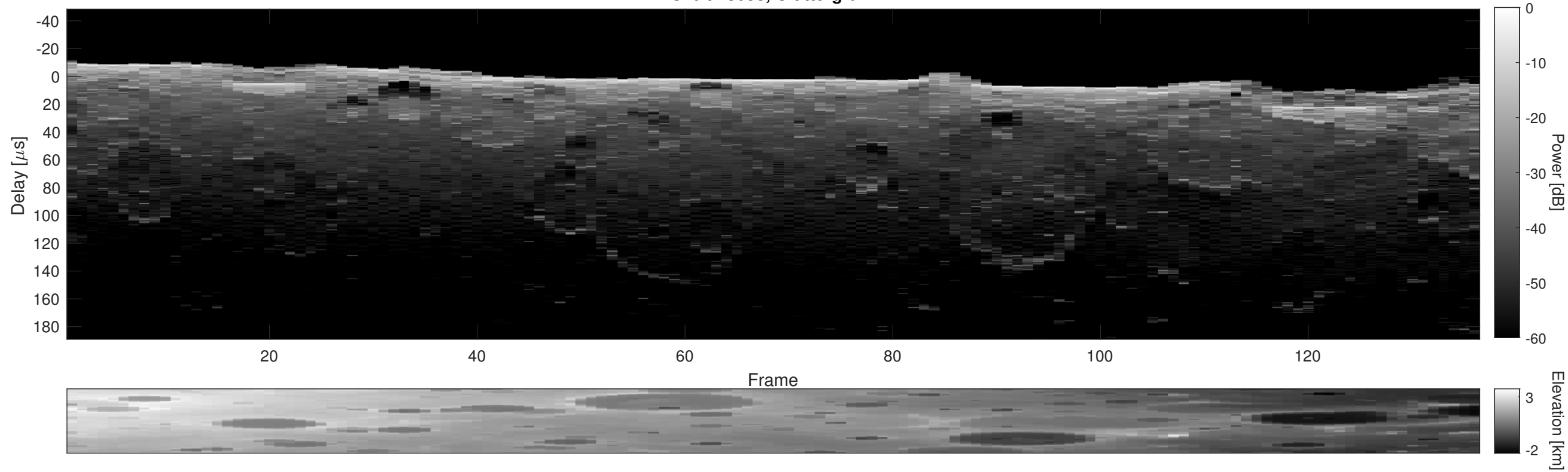
Orbit 13058, Cluttergram
