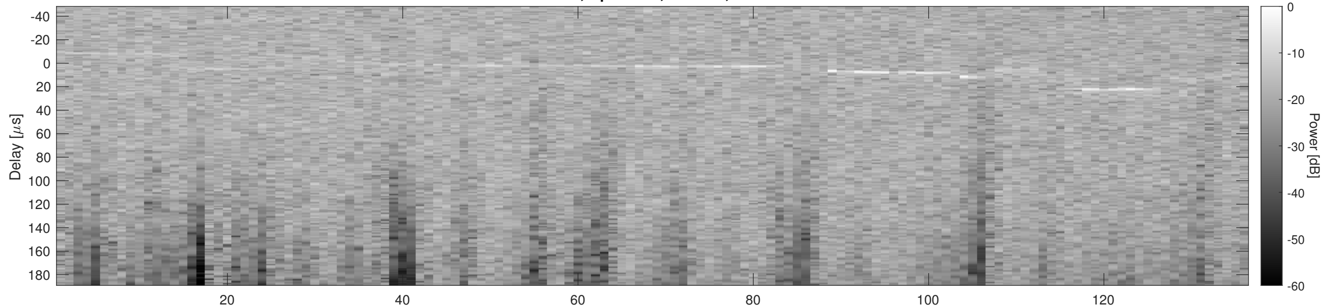
Orbit 13058, Optimized, Window, Channel 2
