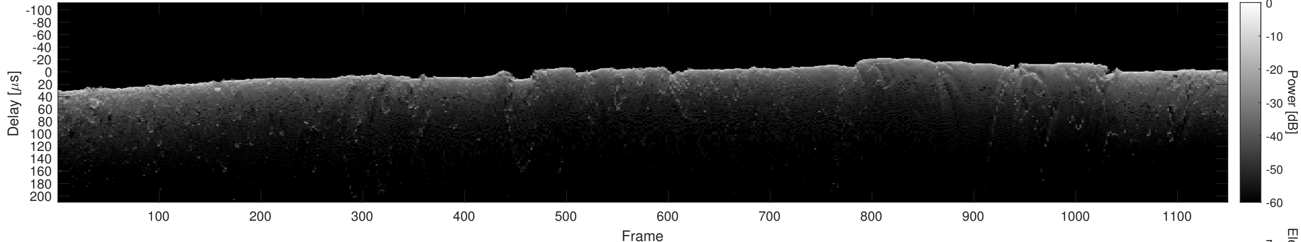
Orbit 13059, Cluttergram
