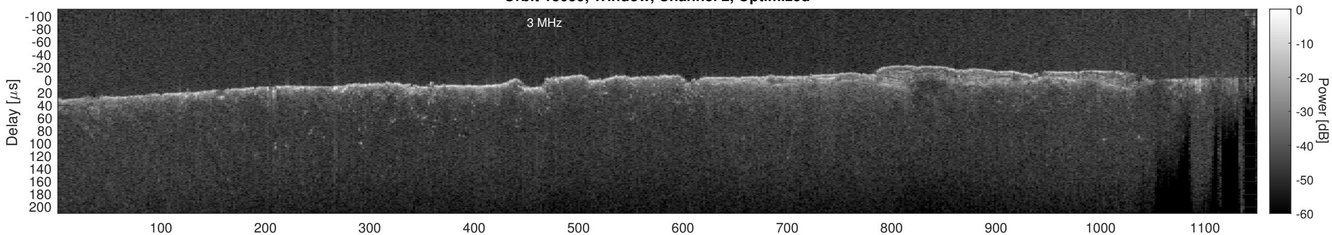
Orbit 13059, Cluttergram
