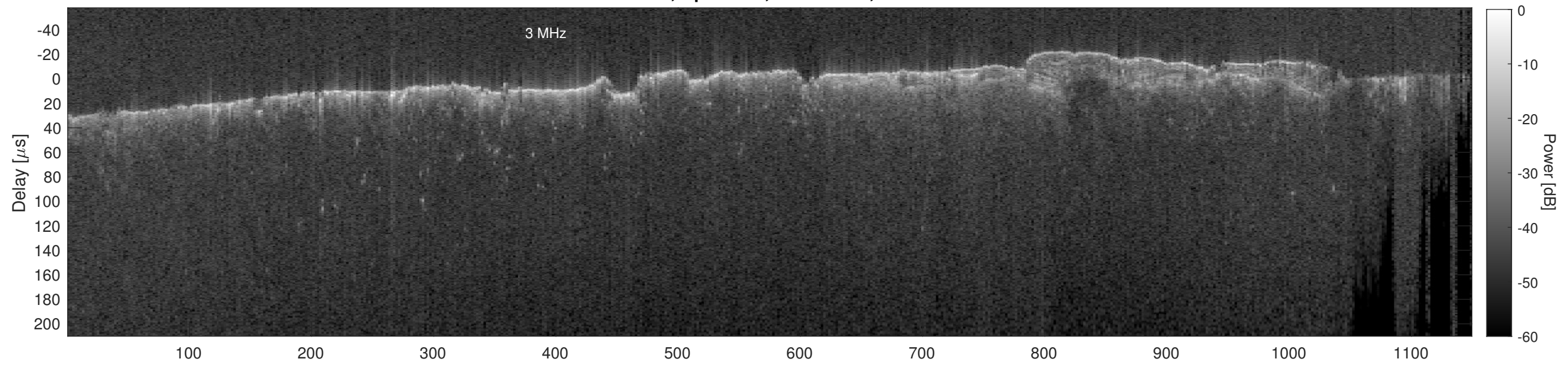
Orbit 13059, Cluttergram
