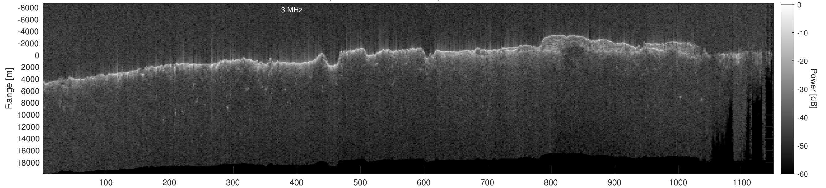
Orbit 13059, Depth-Corrected Cluttergram
