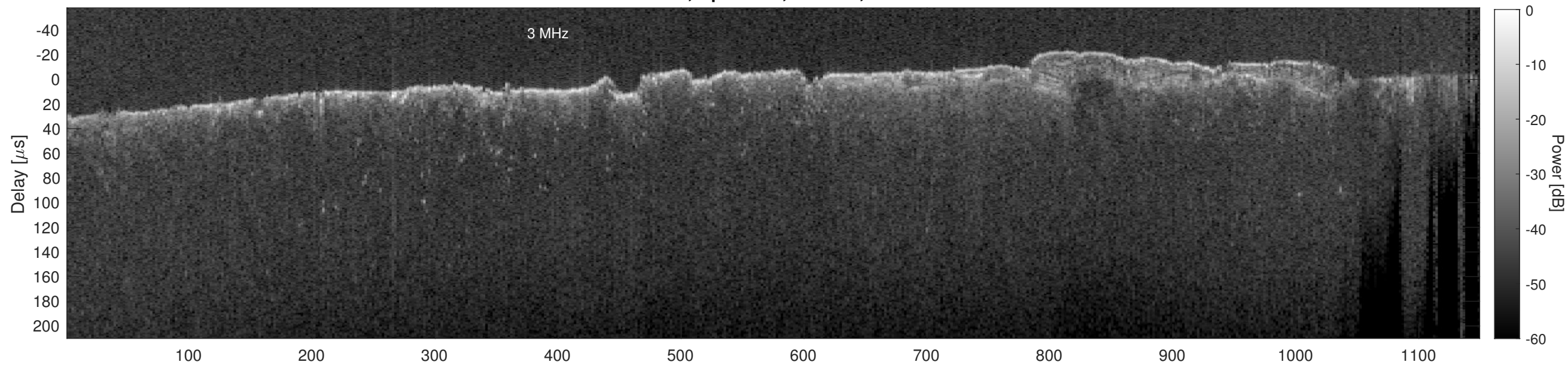
Orbit 13059, Cluttergram
