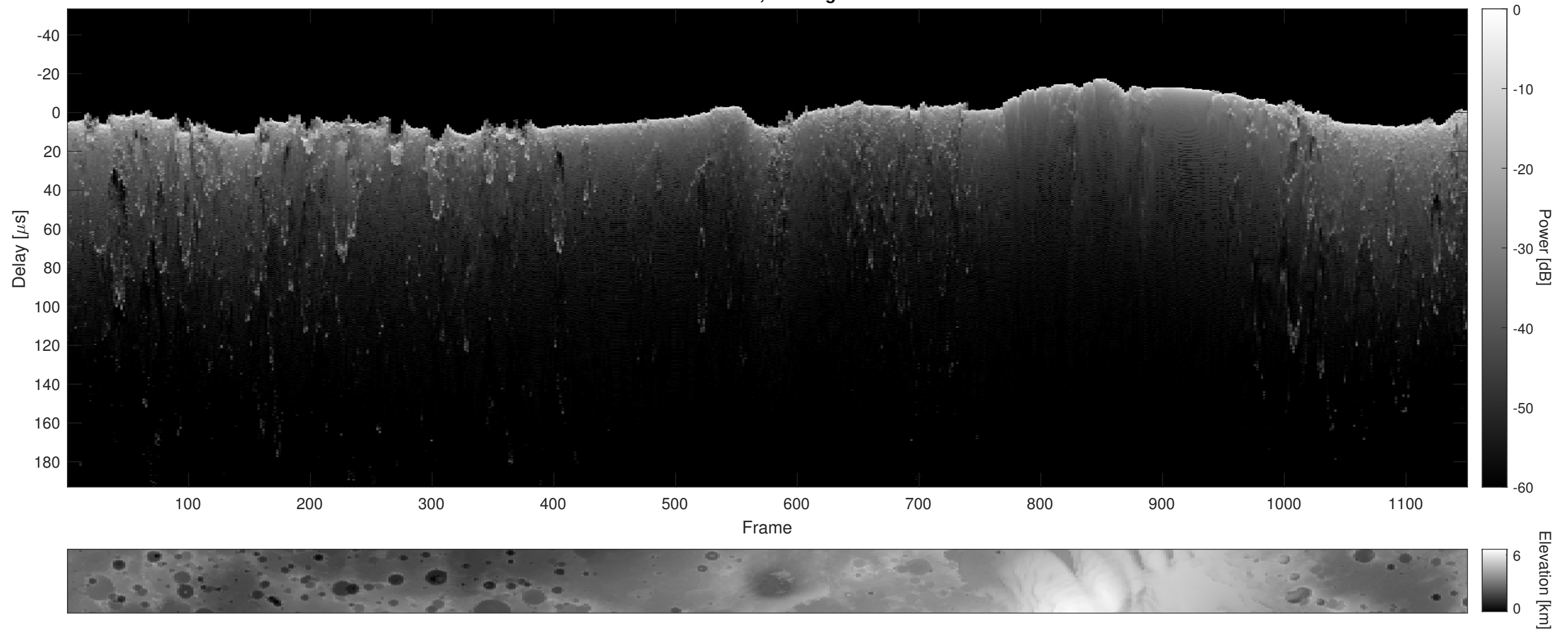
Orbit 13062, Cluttergram
