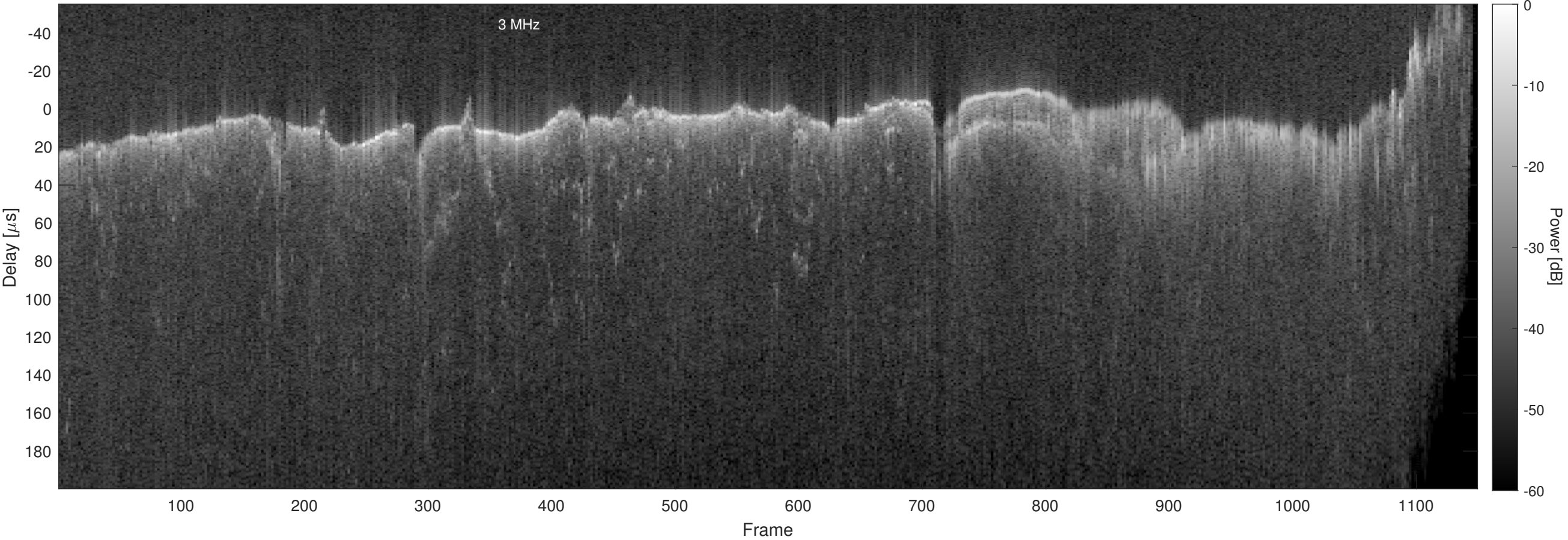
Orbit 13064, Chapman, No Window, Channel 2
