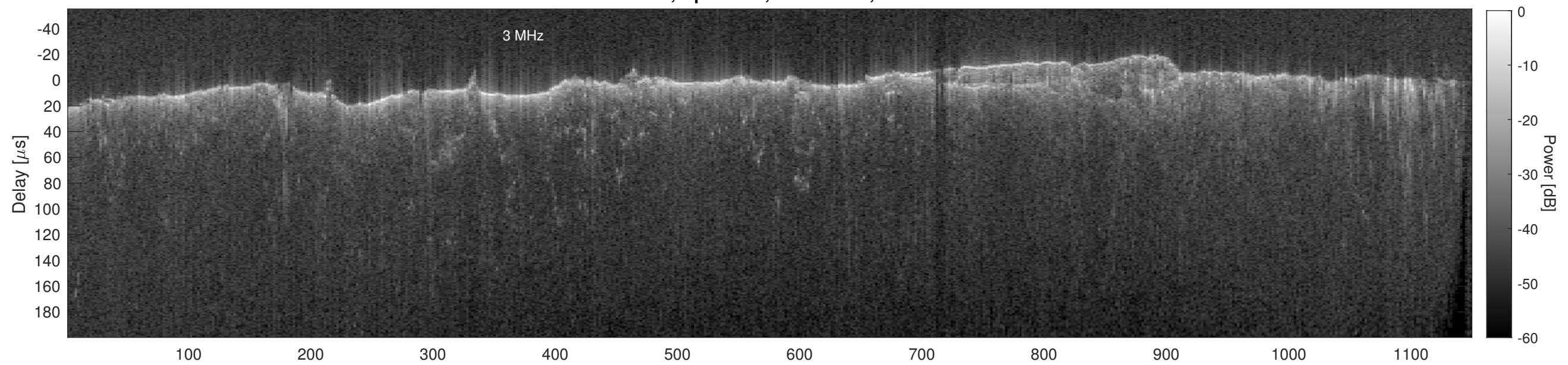
Orbit 13064, Cluttergram
