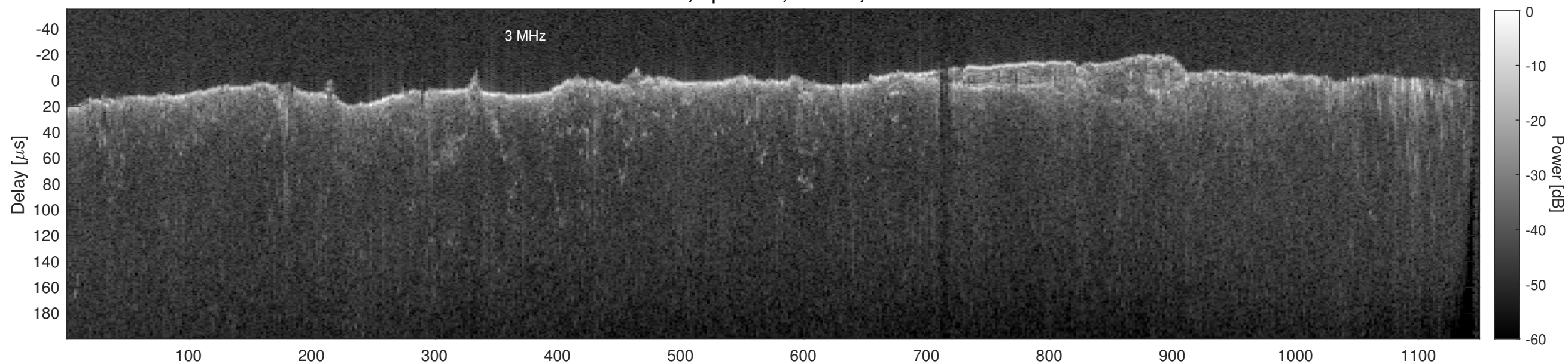
Orbit 13064, Cluttergram
