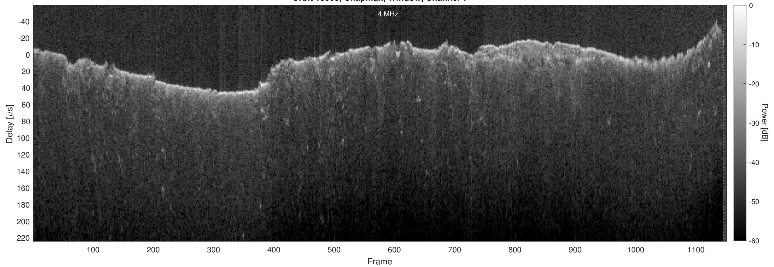
Orbit 13065, Chapman, Window, Channel 2
