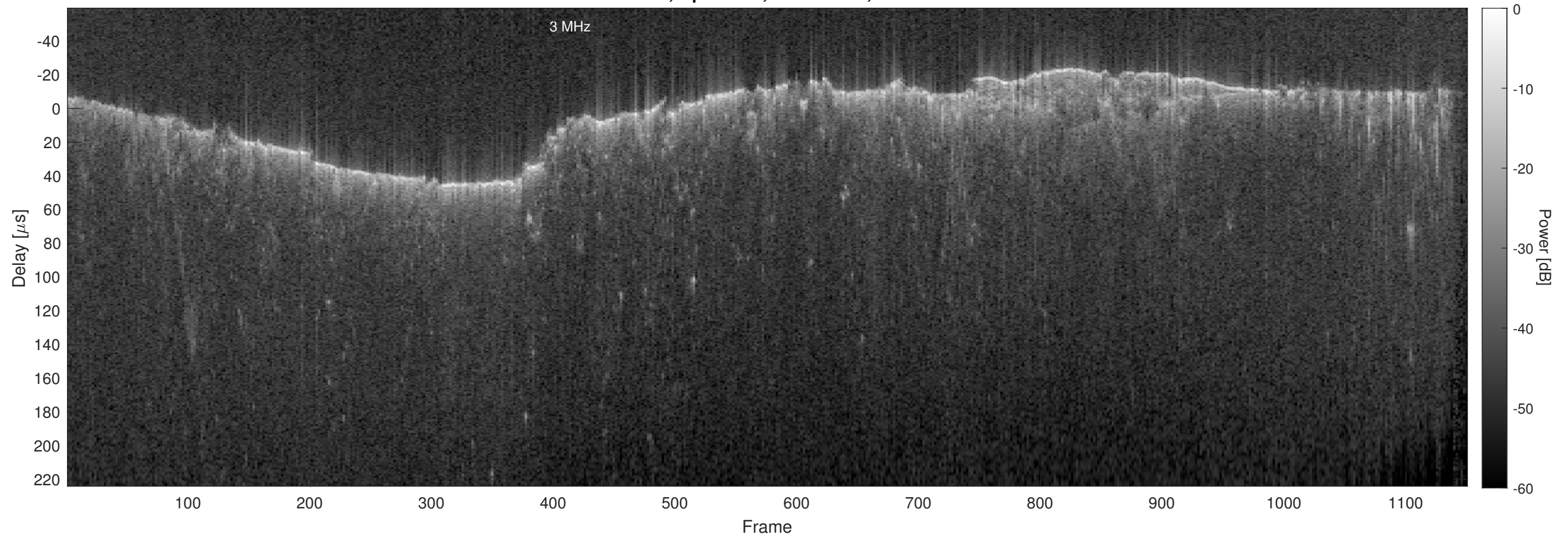
Orbit 13065, Optimized, No Window, Channel 2
