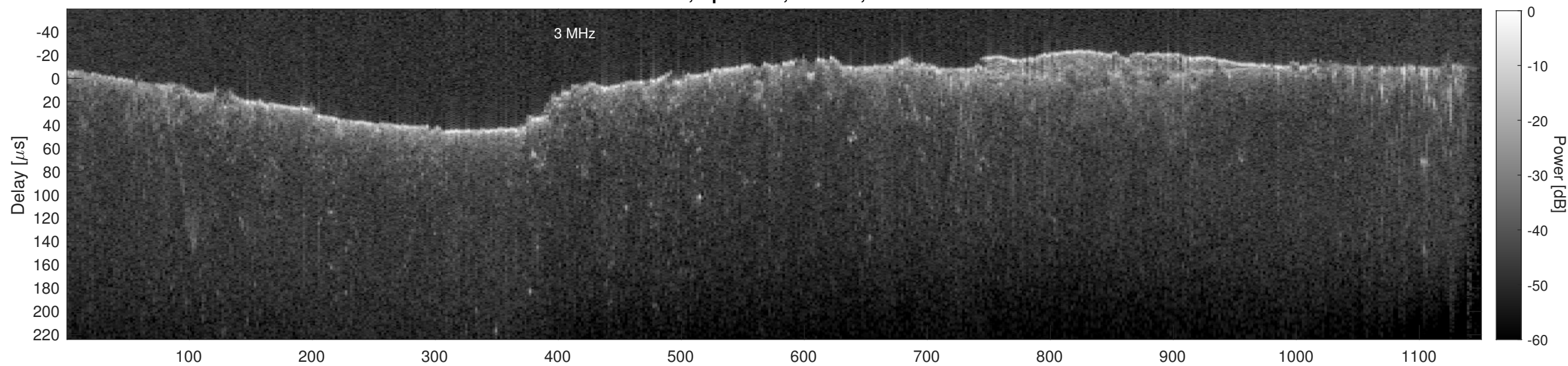
Orbit 13065, Cluttergram
