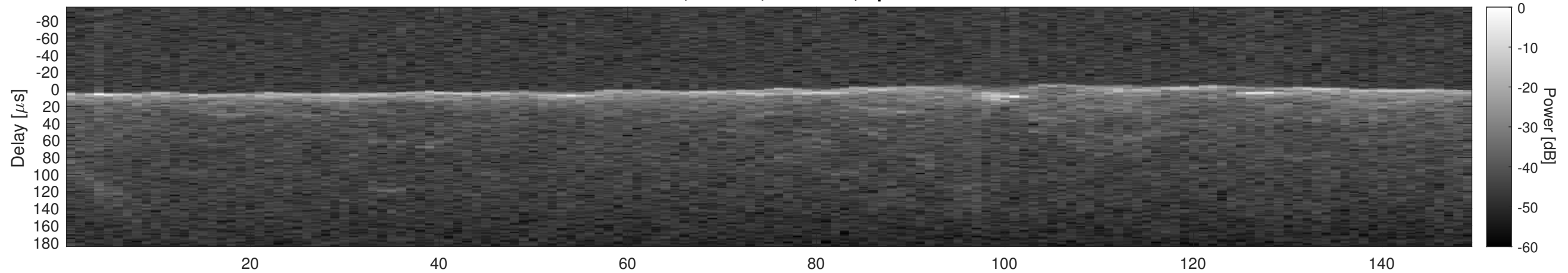
Orbit 13068, Cluttergram
