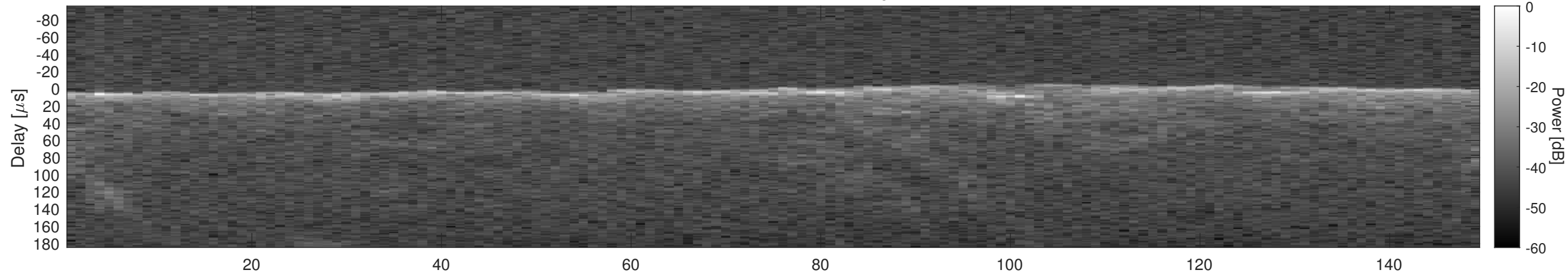
Orbit 13068, Cluttergram
