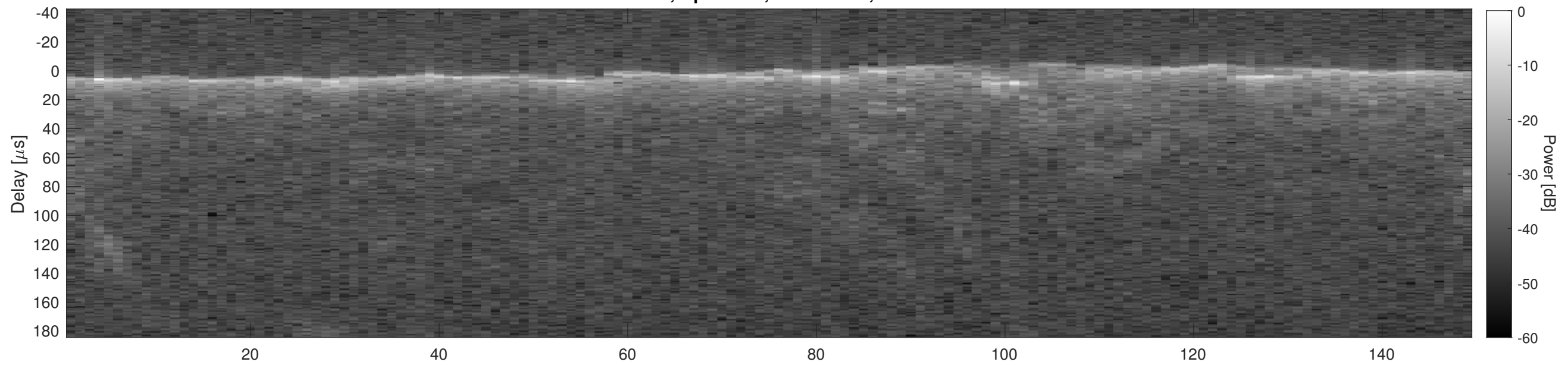
Orbit 13068, Cluttergram
