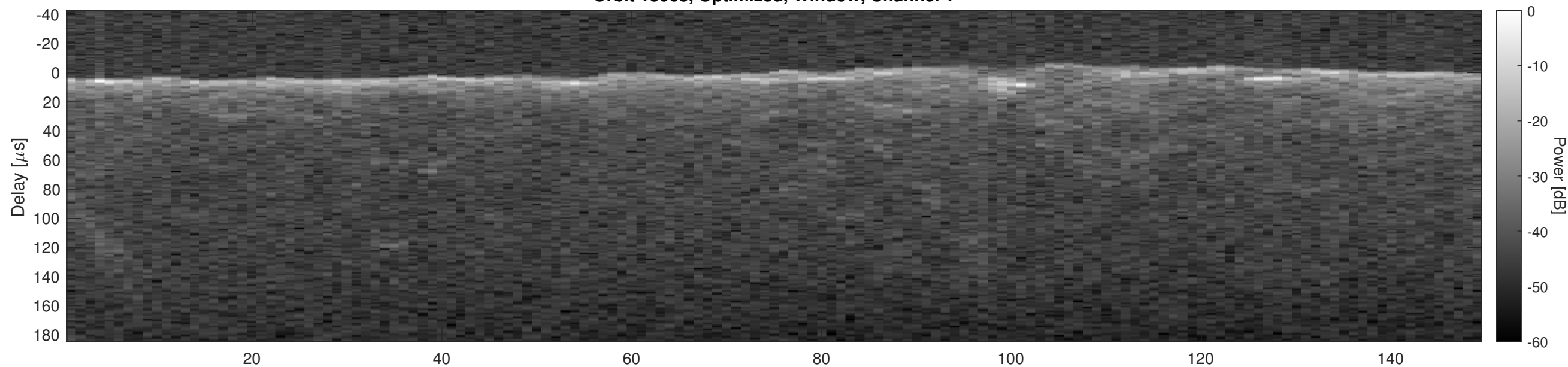
Orbit 13068, Optimized, Window, Channel 2
