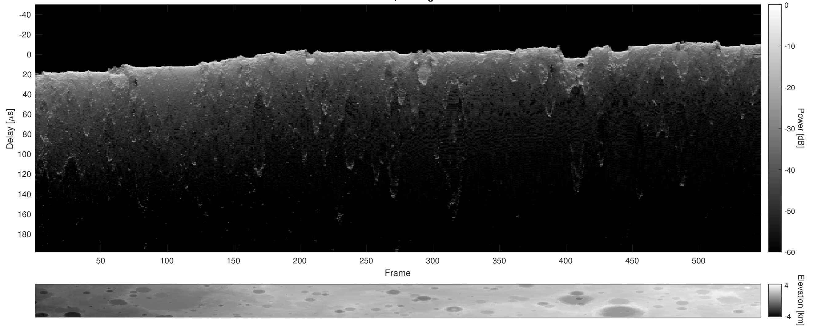
Orbit 13080, Cluttergram
