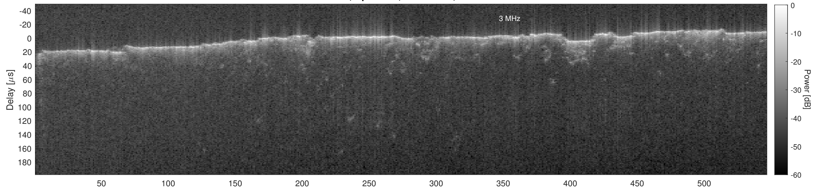
Orbit 13080, Cluttergram
