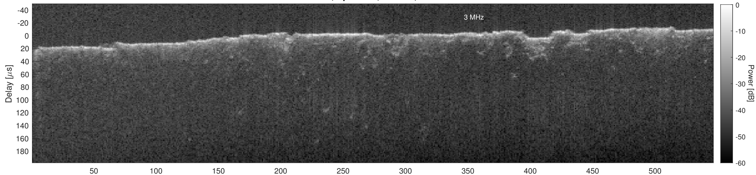
Orbit 13080, Cluttergram
