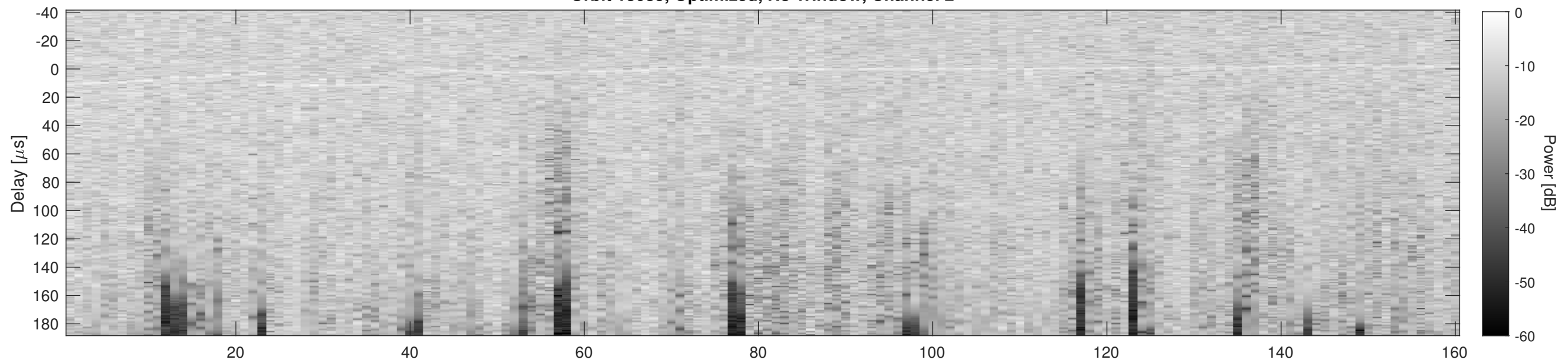
Orbit 13085, Cluttergram
