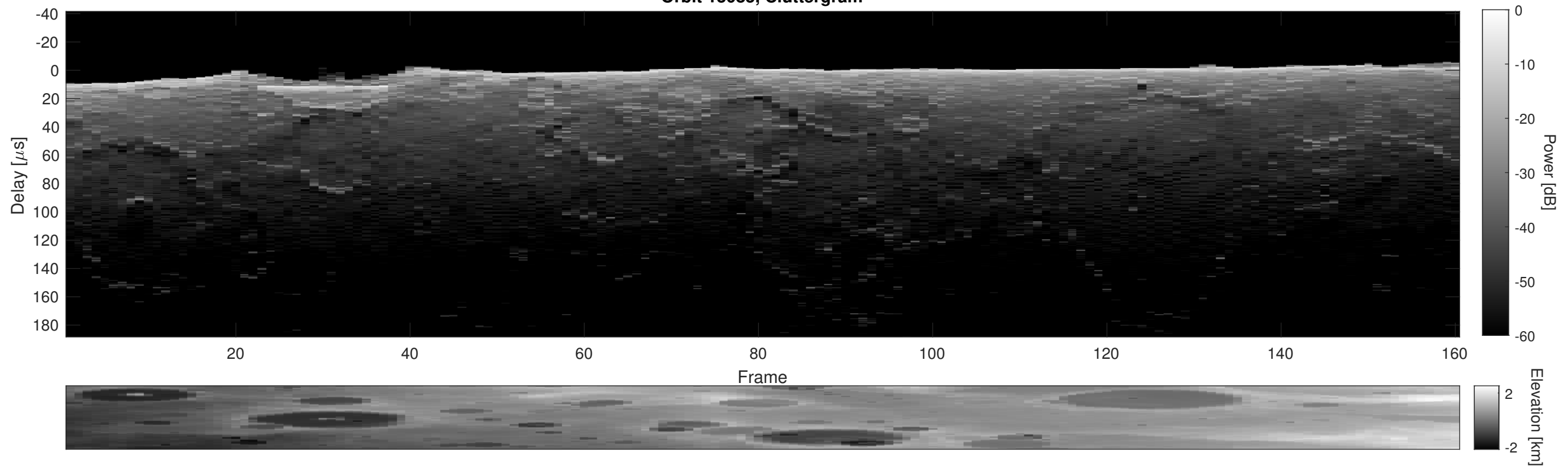
Orbit 13085, Cluttergram
