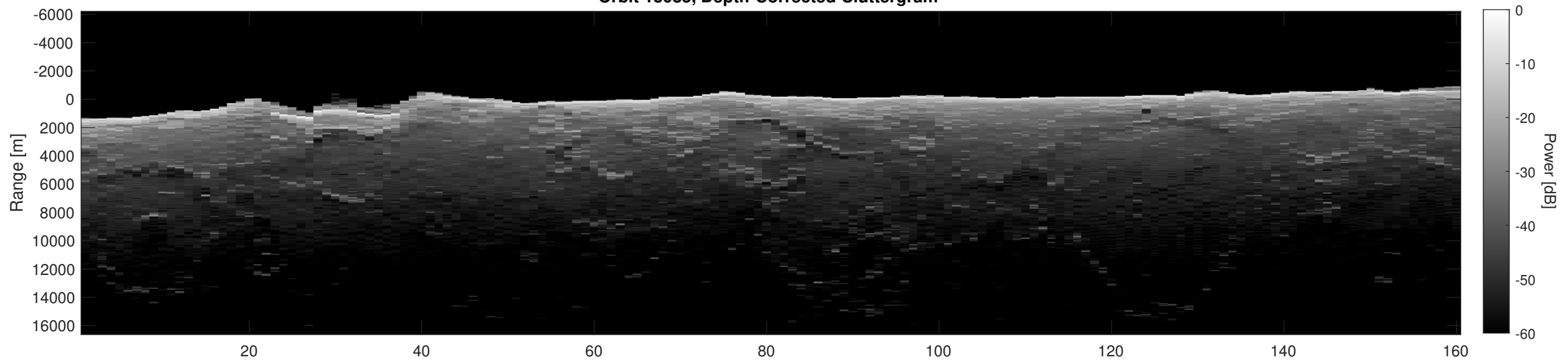
Orbit 13085, Depth-Corrected Cluttergram
