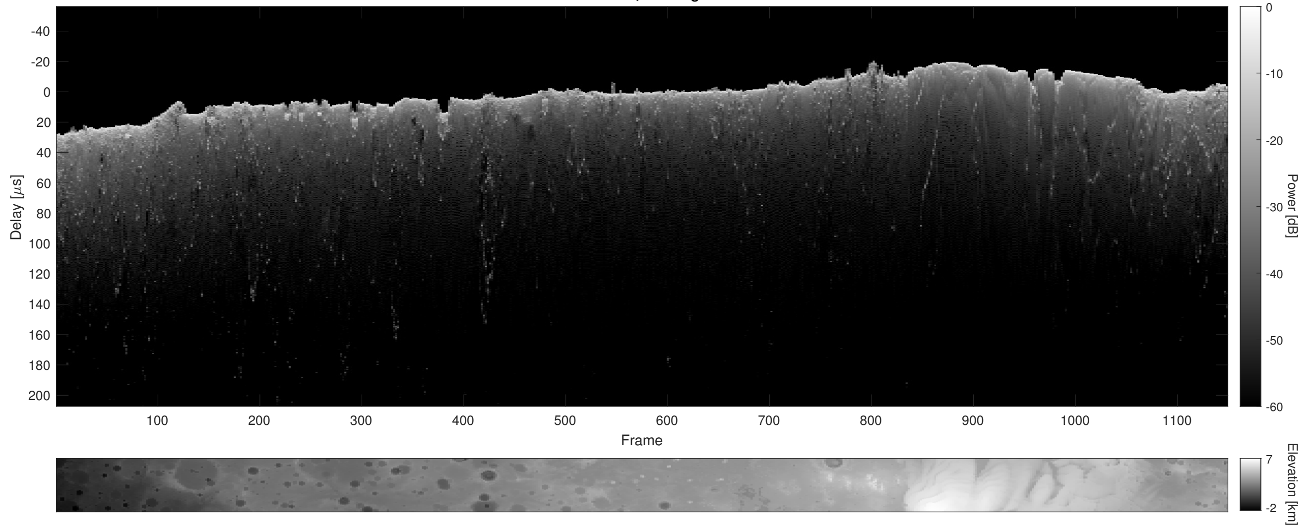
Orbit 13087, Cluttergram
