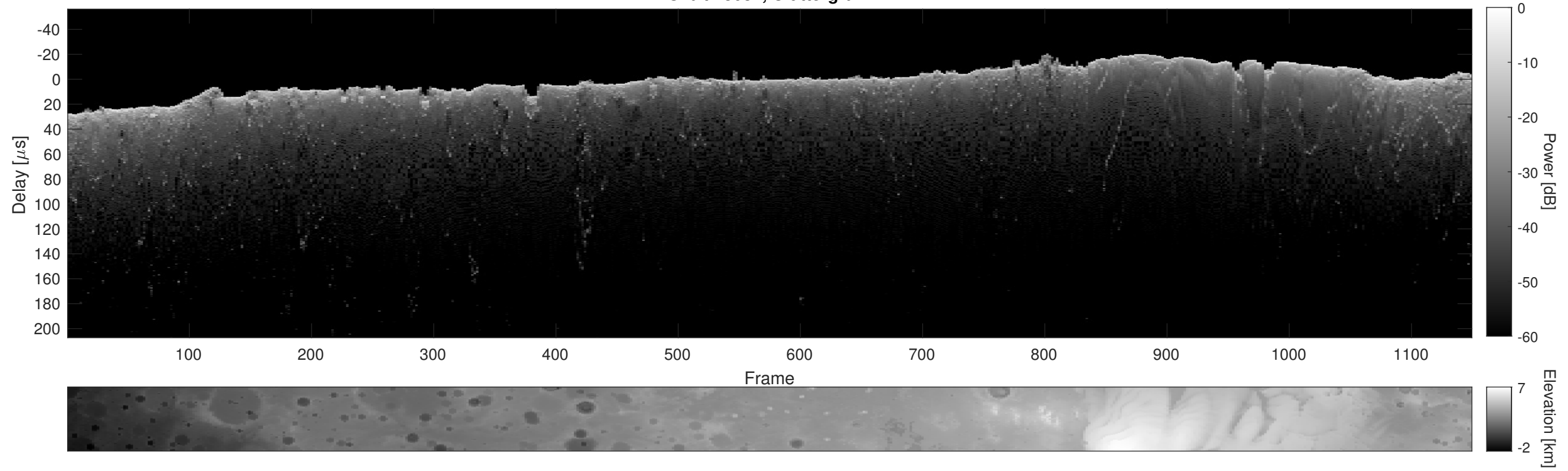
Orbit 13087, Cluttergram
