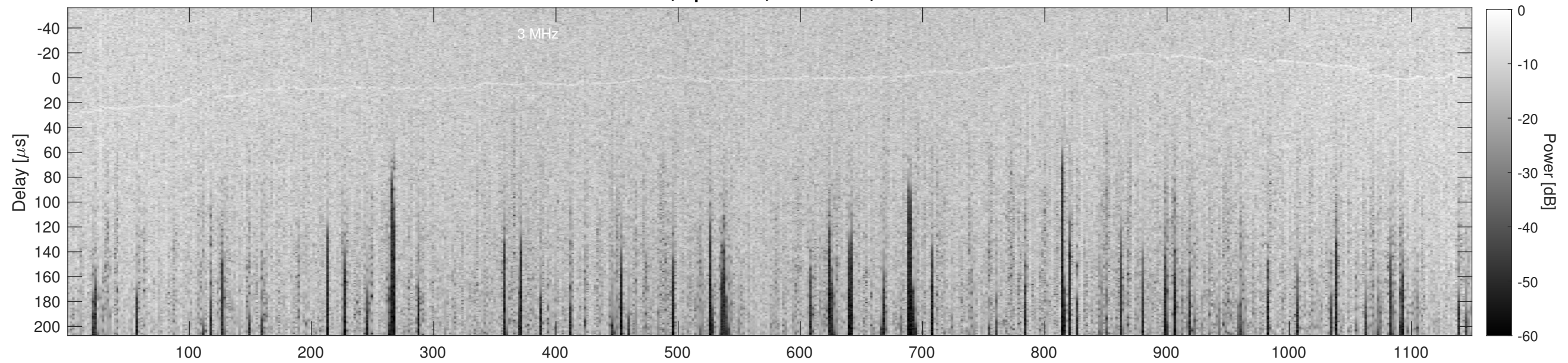
Orbit 13087, Cluttergram
