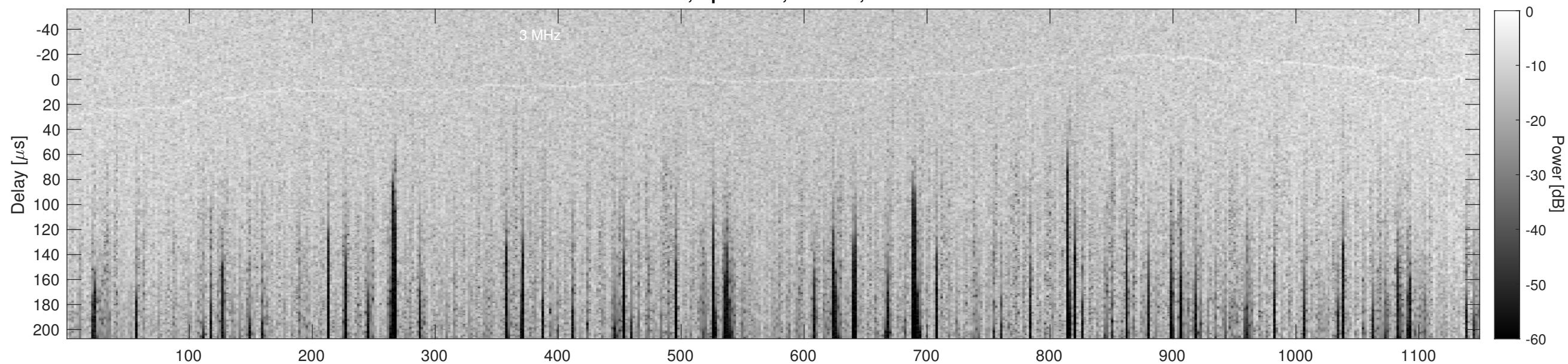
Orbit 13087, Cluttergram
