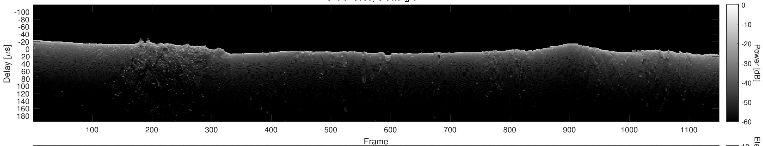
Orbit 13088, Cluttergram
