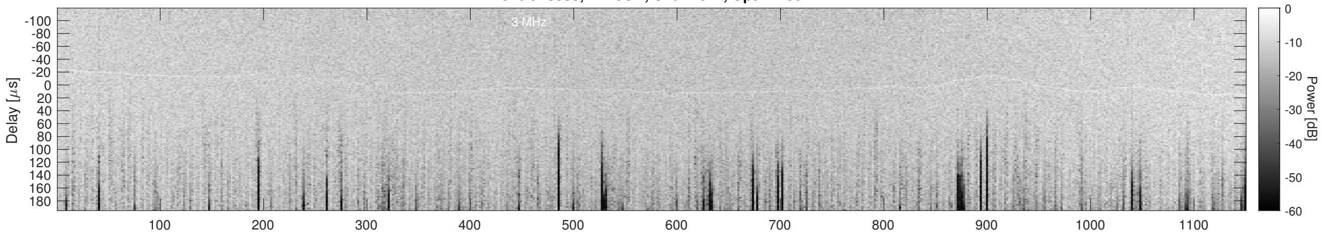
Orbit 13088, Cluttergram
