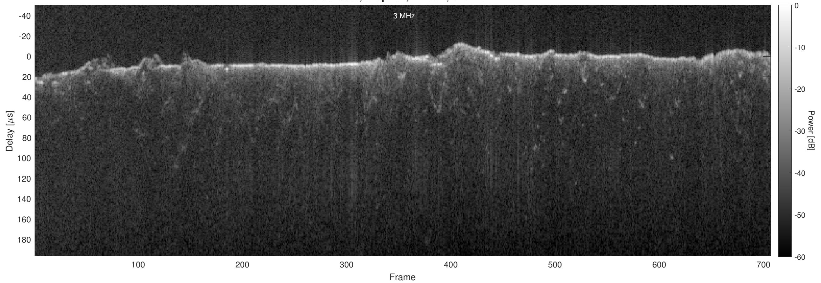
Orbit 13099, Chapman, Window, Channel 2
