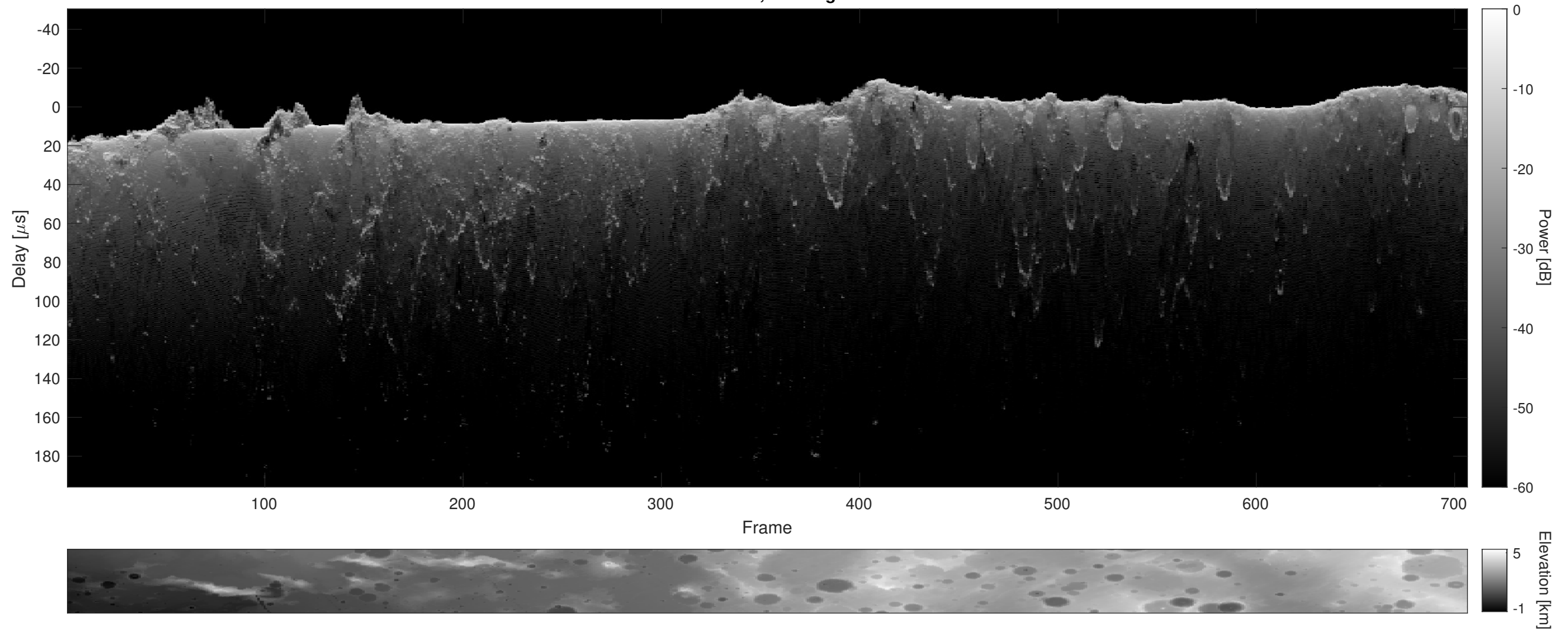
Orbit 13099, Cluttergram
