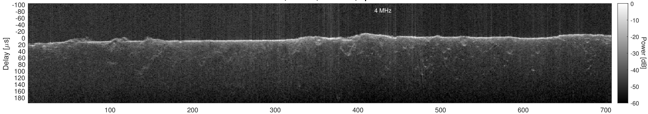
Orbit 13099, Cluttergram
