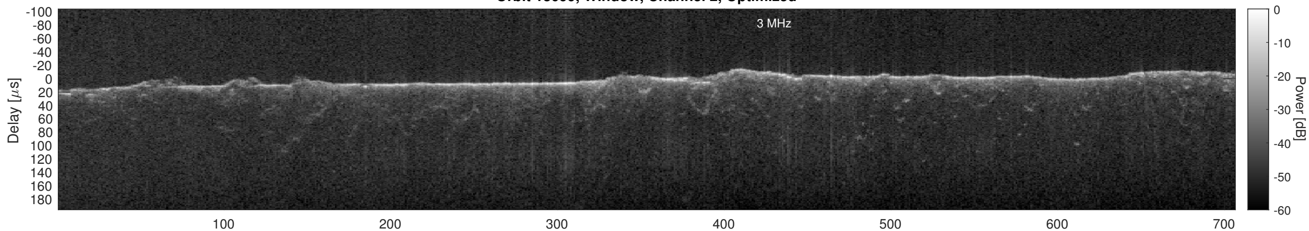
Orbit 13099, Cluttergram
