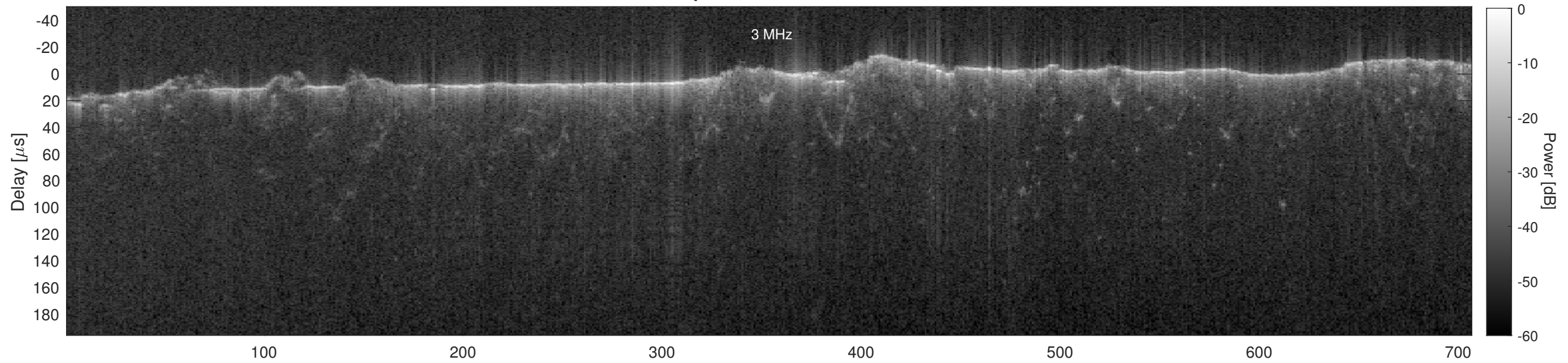
Orbit 13099, Cluttergram
