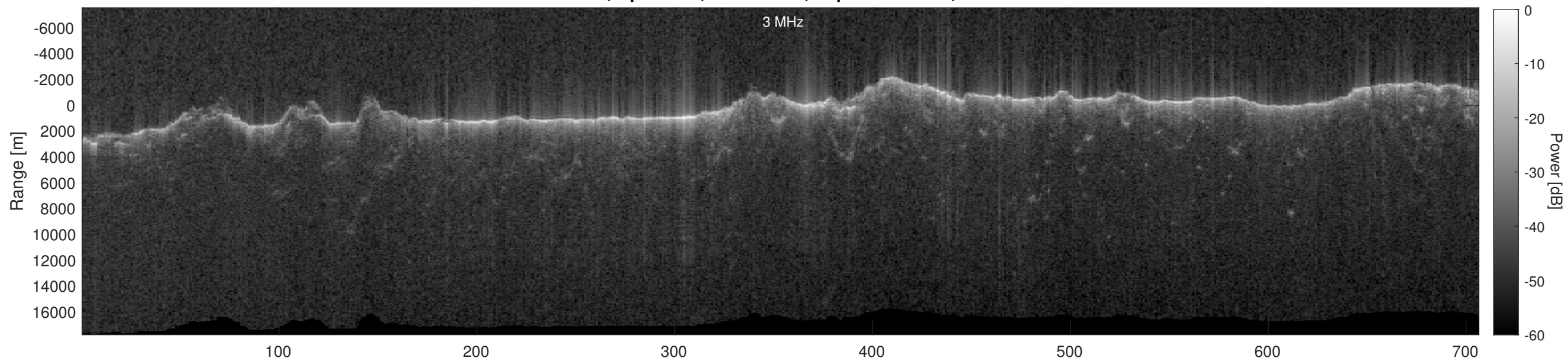
Orbit 13099, Depth-Corrected Cluttergram
