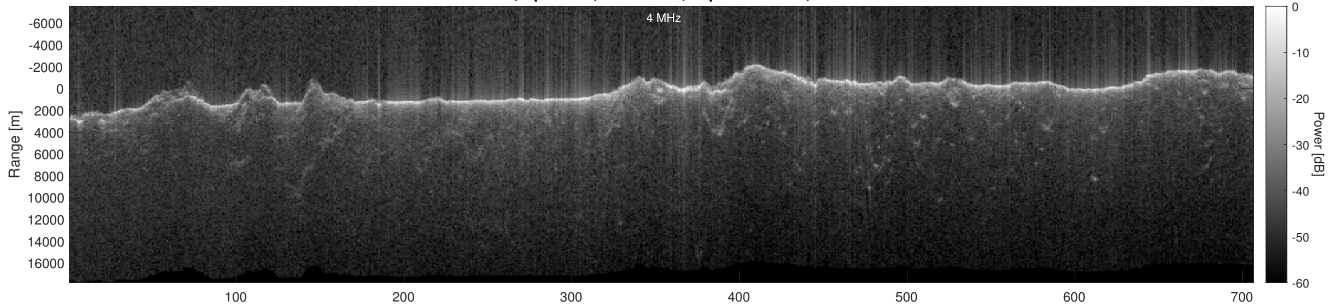
Orbit 13099, Optimized, No Window, Depth-Corrected, Channel 2
