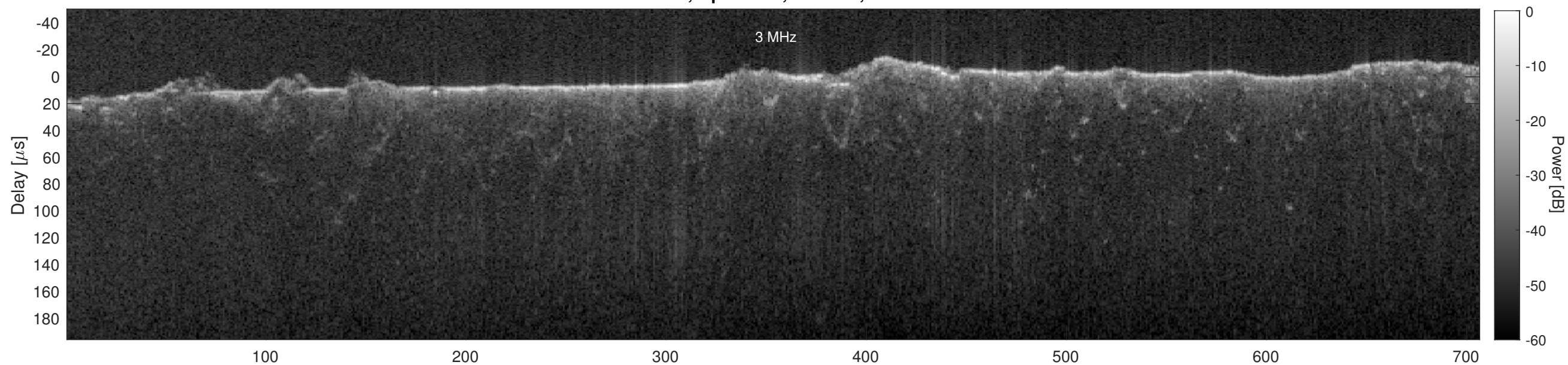
Orbit 13099, Cluttergram
