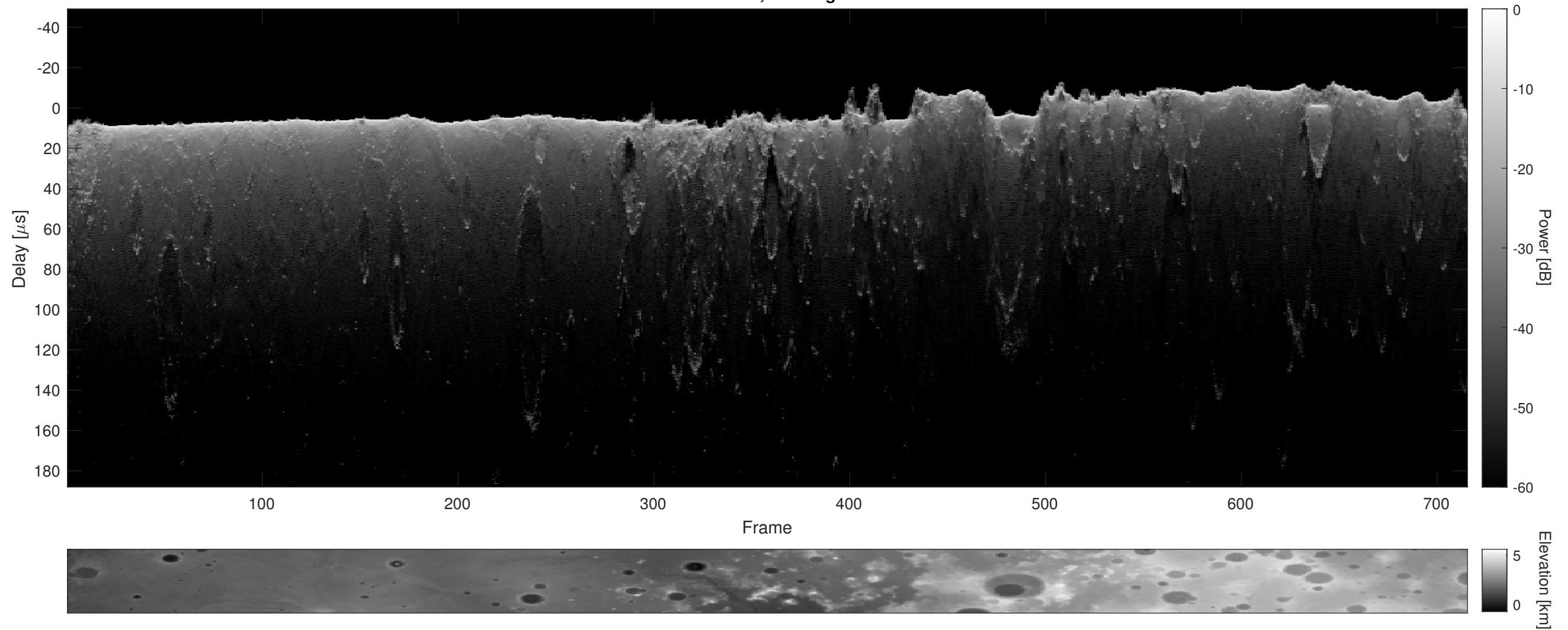
Orbit 13100, Cluttergram
