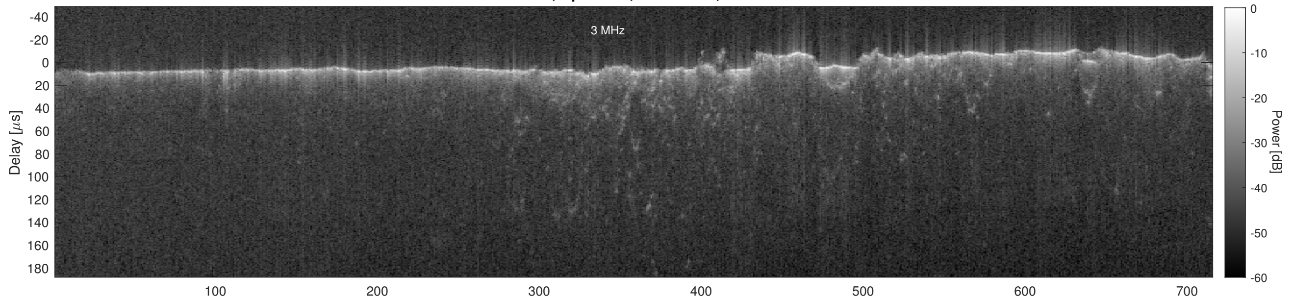
Orbit 13100, Cluttergram
