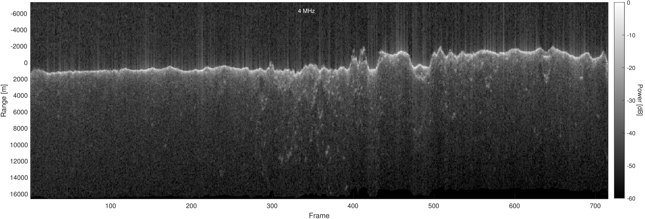
Orbit 13100, Optimized, No Window, Depth-Corrected, Channel 2
