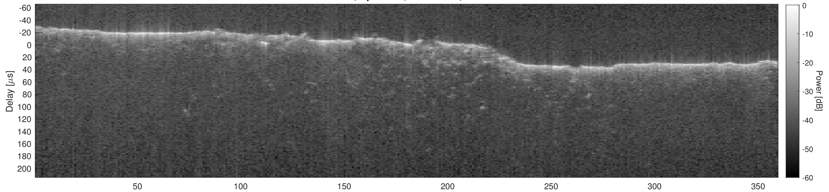
Orbit 13104, Cluttergram
