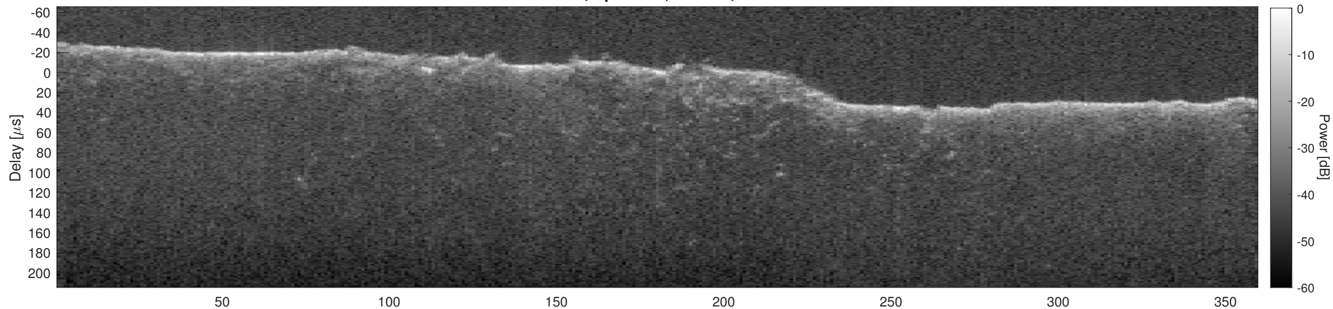
Orbit 13104, Cluttergram
