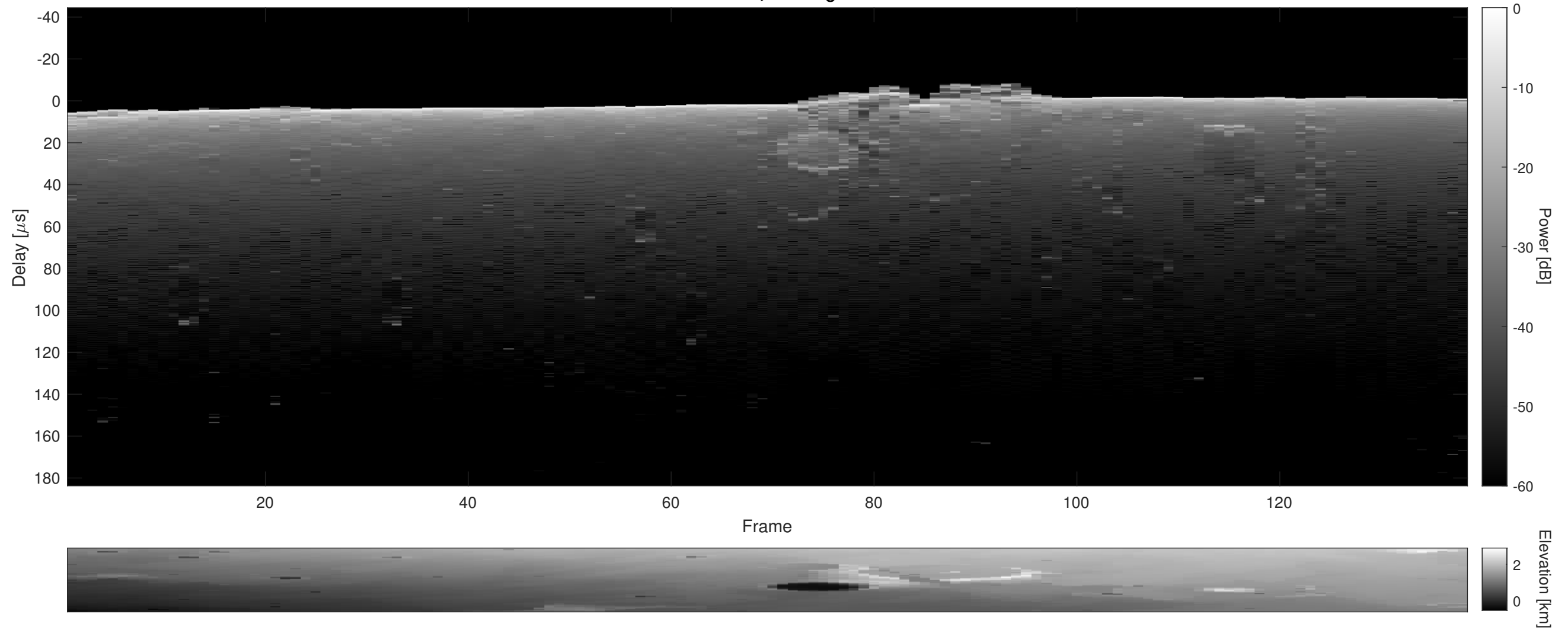
Orbit 13106, Cluttergram
